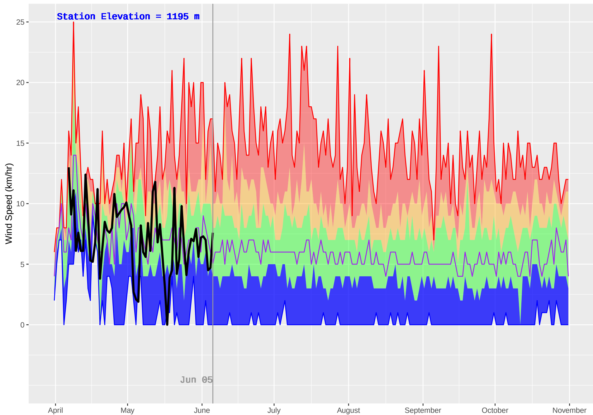
VALEMOUNT 2 (200) : Historical (1986–2018) and Current (2019) Daily Wind Speed
