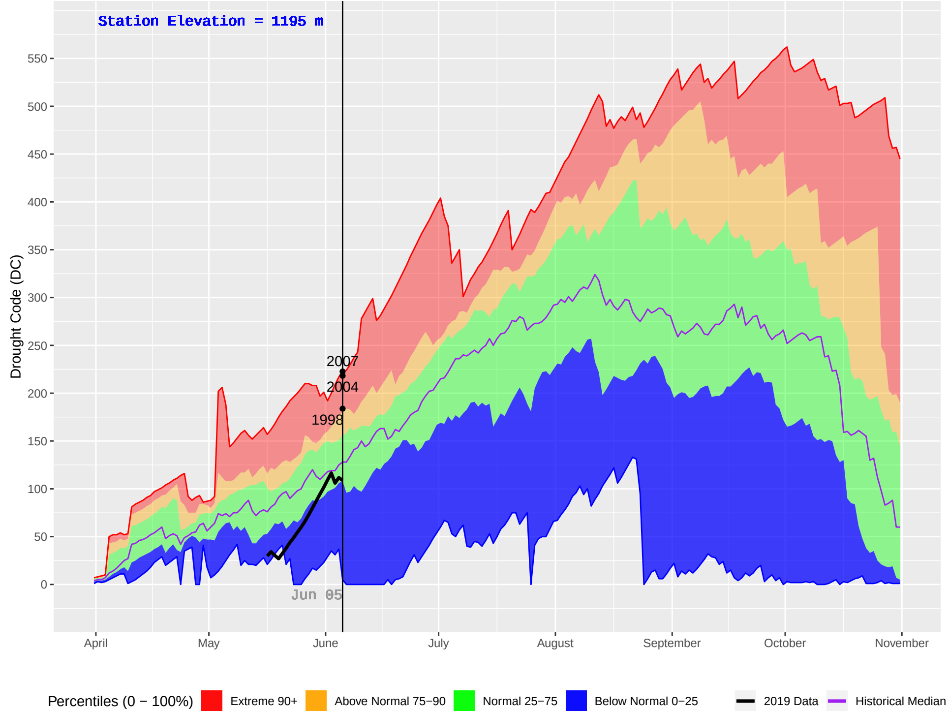
VALEMOUNT 2 (200) : Historical (1986–2018) and Current (2019) Daily Drought Code (DC)
