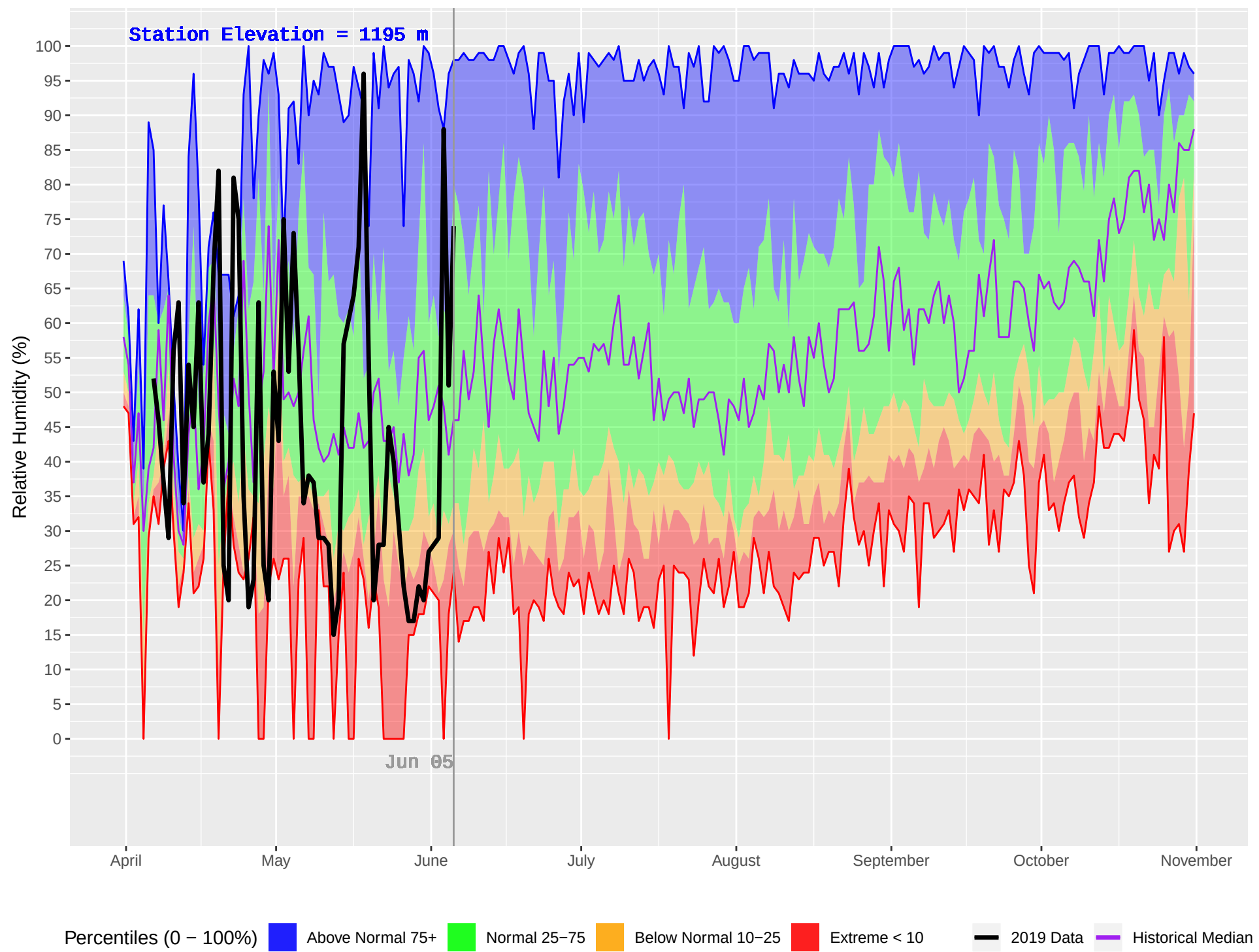
VALEMOUNT 2 (200) : Historical (1986–2018) and Current (2019) Daily Relative Humidity
