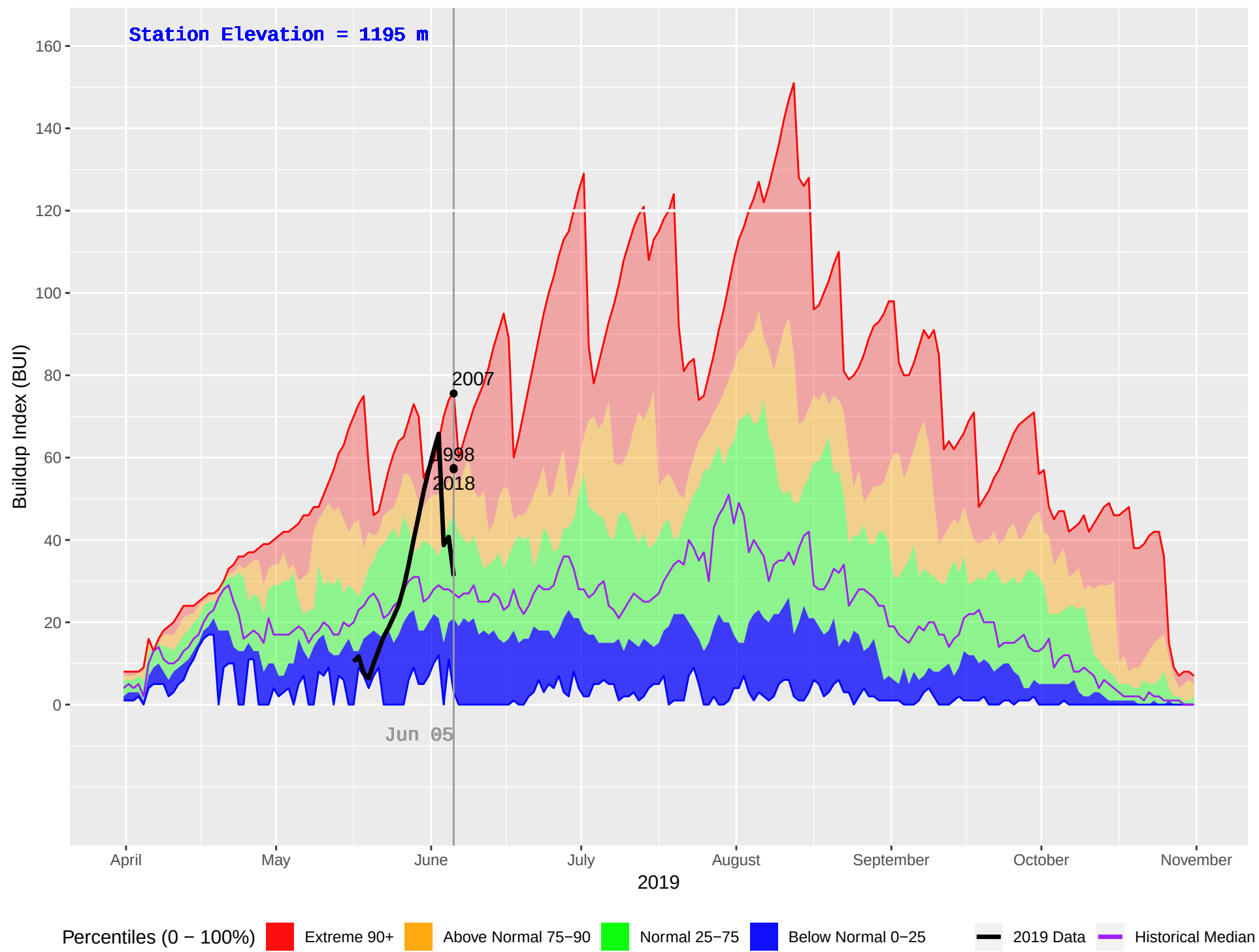
VALEMOUNT 2 (200) : Historical (1986–2018), Current (2019) Daily Buildup Index (BUI)
