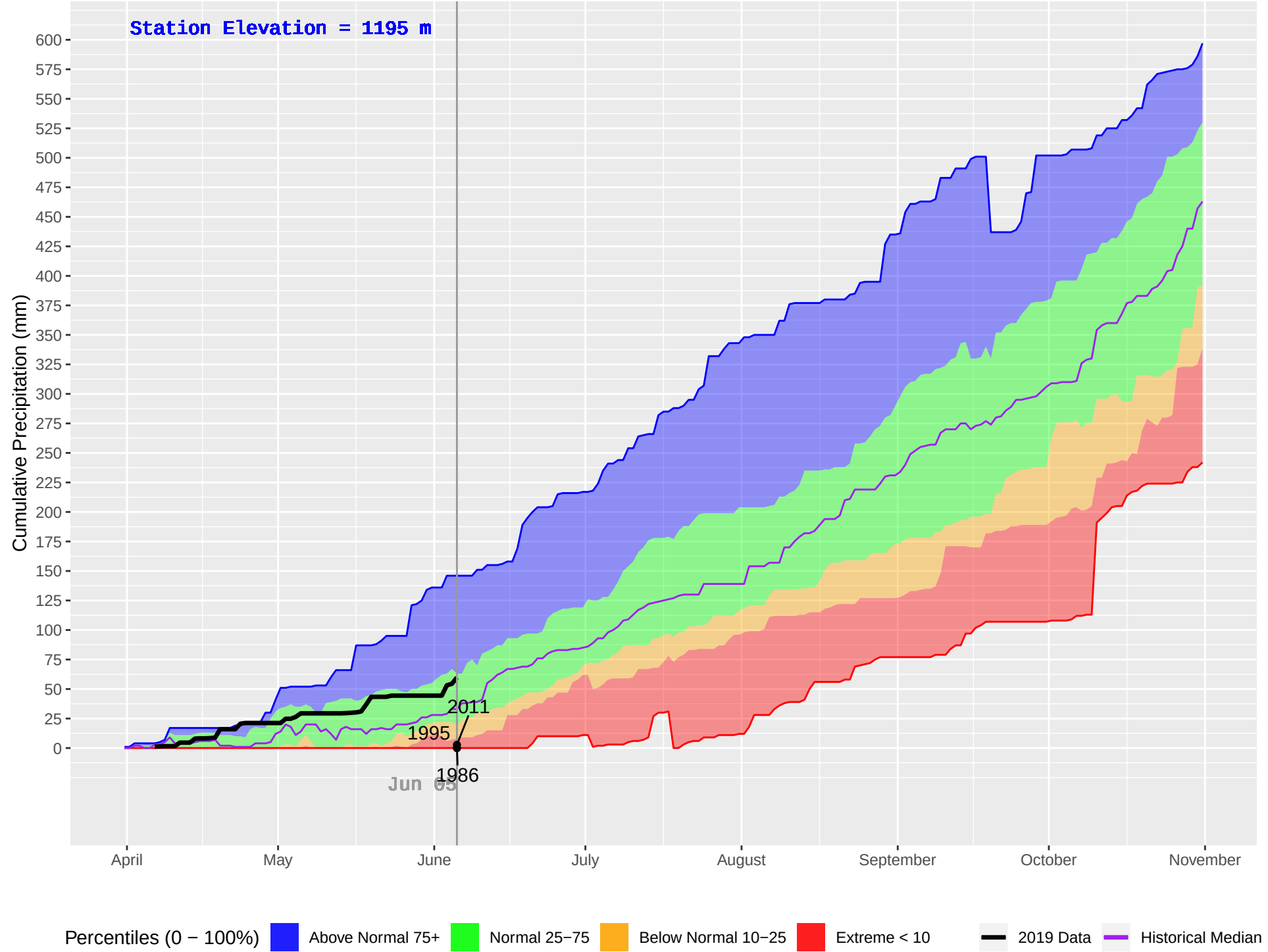
VALEMOUNT 2 (200) : Historical (1986–2018), Current (2019) Daily Cumulative Precipitation
