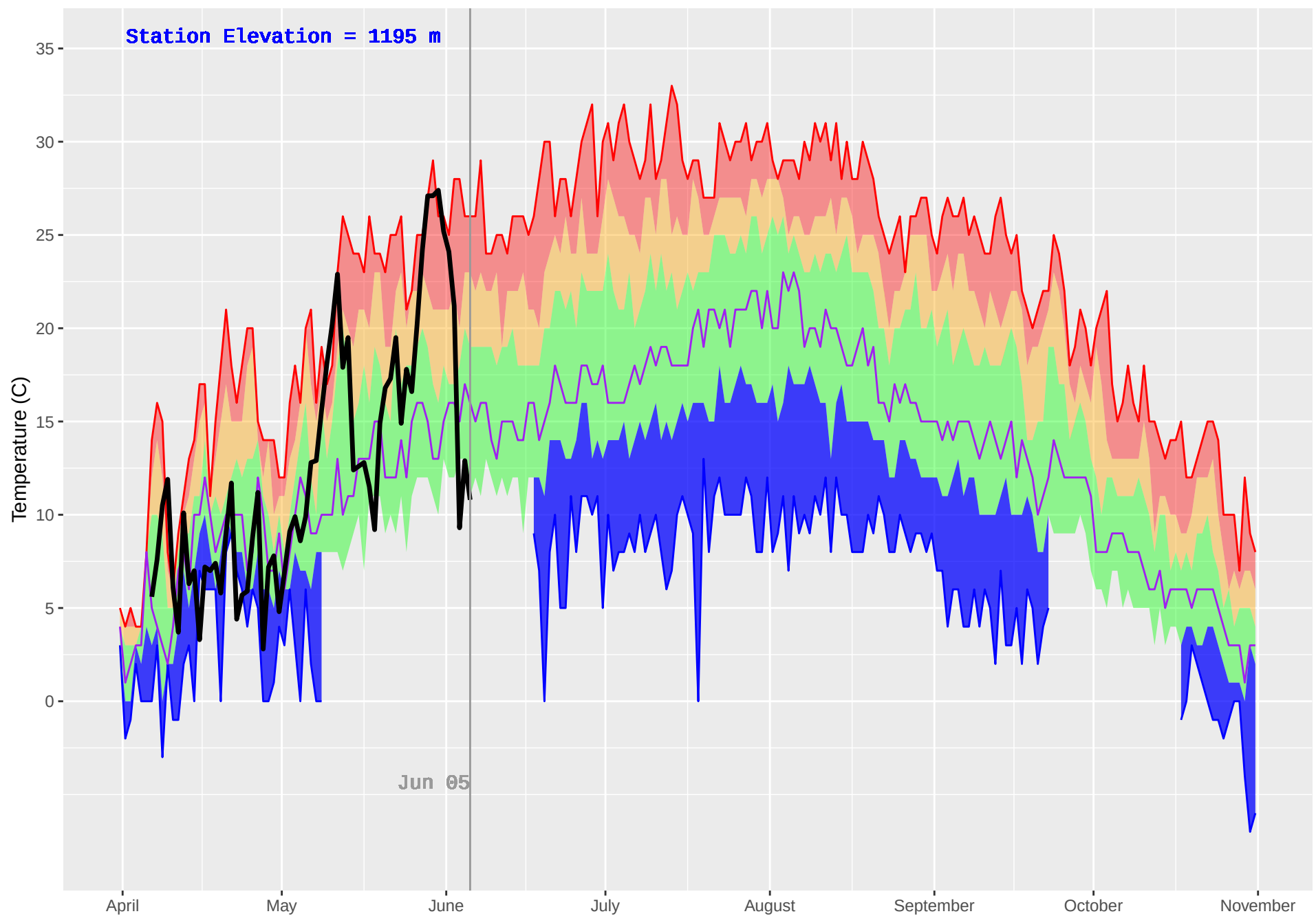
VALEMOUNT 2 (200) : Historical (1986–2018) and Current (2019) Daily Temperature
