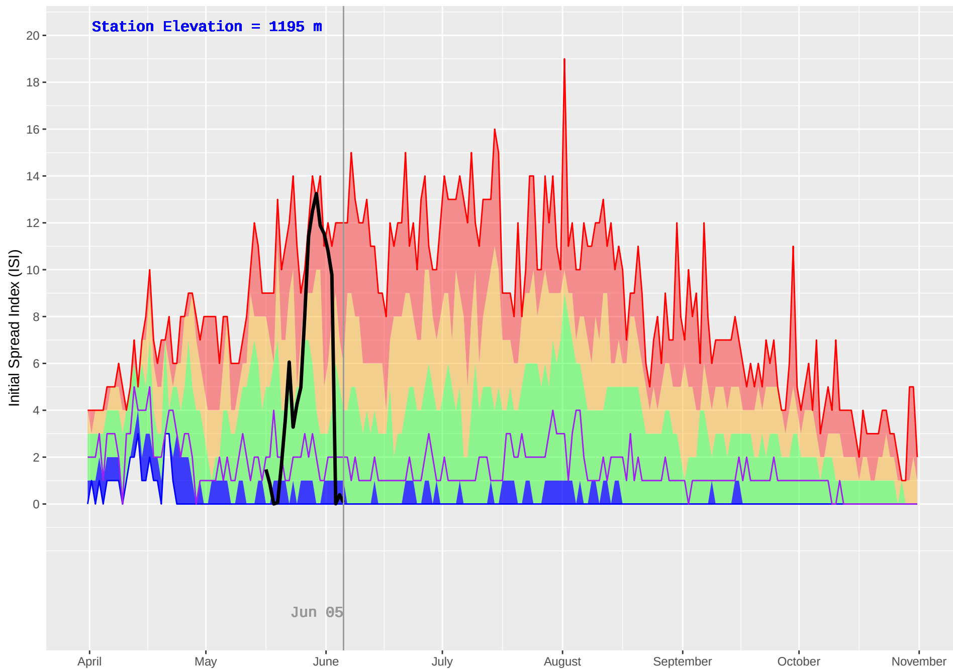
VALEMOUNT 2 (200) : Historical (1986–2018) and Current (2019) Daily Initial Spread Index (ISI)
