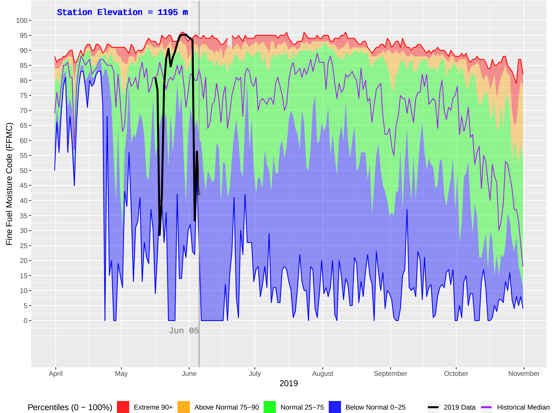
VALEMOUNT 2 (200) : Historical (1986–2018) and Current (2019) Daily Fine Fuel Moisture Code (FFMC)
