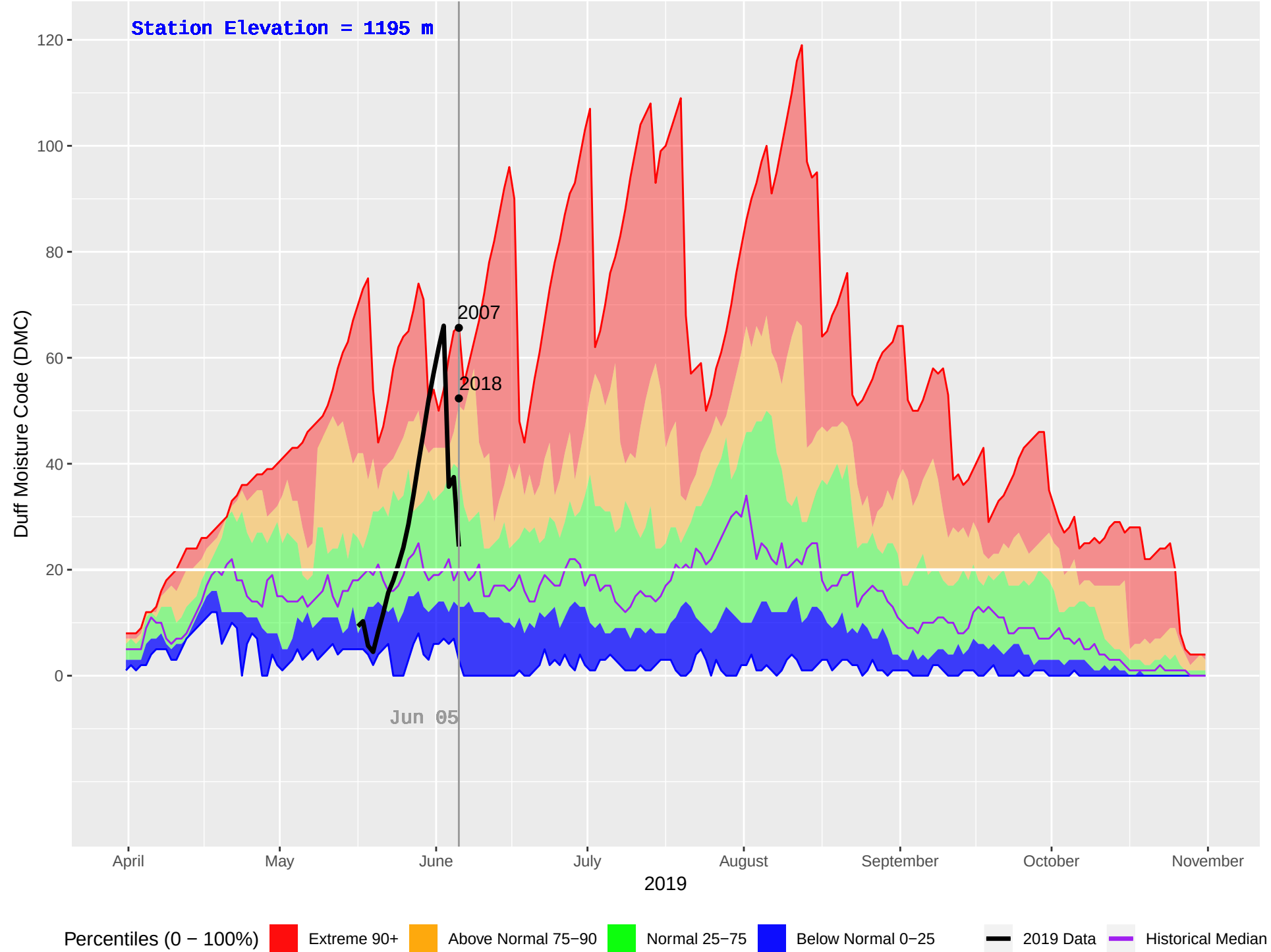
VALEMOUNT 2 (200) : Historical (1986–2018), Current (2019) Daily Duff Moisture Code (DMC)
